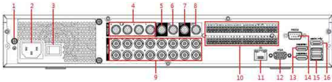
Figure 3-18
